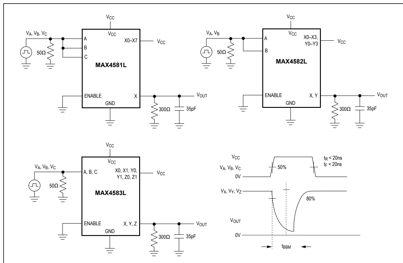
Figure 3. Break-Before-Make Interval
