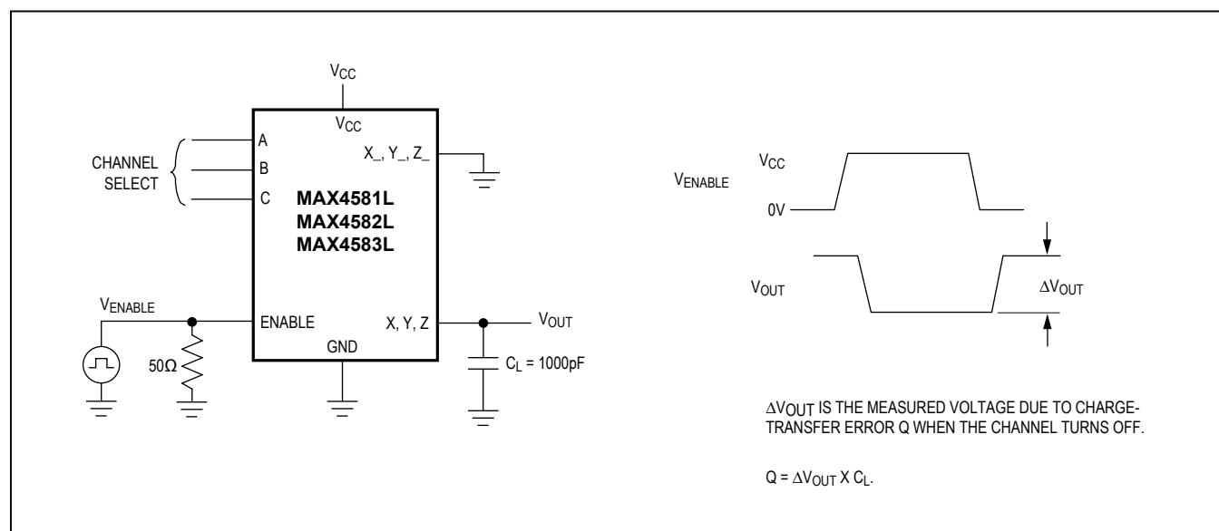
Figure 4. Charge Injection
